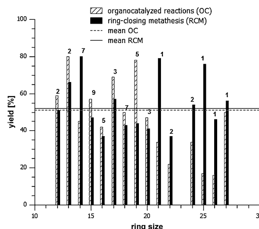
Figure 1. Mean yields with respect to ring size for organocatalysis and ring-closing metathesis steps. Numbers above the bars represent the number of macrocycles of the corresponding ring size in the library.
