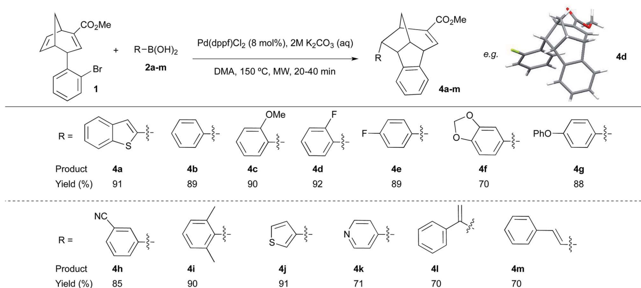
Scheme 2 Domino Heck–Suzuki reactions of boronic acids 2a–m with bicyclo[3.2.1]octadiene 1 to form compounds 4a–m. MW = microwave irradiation. 2 equivalents of boronic coupling partner (2a–m) were used in all reactions. Yields of isolated products given in all cases. X-ray crystal structure of compound 4d shown.
